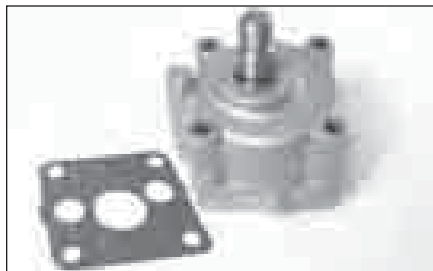
Pump, Oil w/gasket (CT4 engines, except 91) Order Part #: P-25-37040-00-B (Replaces Carrier #: 25-37040-00)
