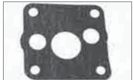
Gasket, Oil Pump (CT4 engines, except 91) Order Part #: P-25-37041-00 (Replaces Carrier #: 25-37041-00)
