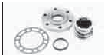
Seal, Shaft (05D) Order Part #: P-17-44135-00 (Replaces Carrier #: 17-44135-00)
