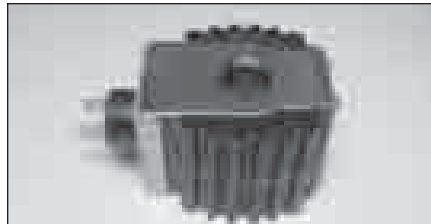
Coil, Solenoid (SV-3) Order Part #: P-14-00145-03 (Replaces Carrier #: 14-00145-03)
