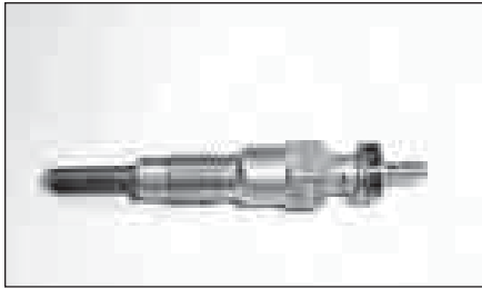
Plug, Glow (M8 Fast Glow) (91TV and 69TV) Order Part #: P-25-15330-00 (Replaces Carrier #: 25-15330-00)
