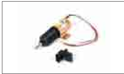
Solenoid, Fuel c/w connector OrderPart# 30-122-05K (Replaces Carrier #: 30-122-05K)
